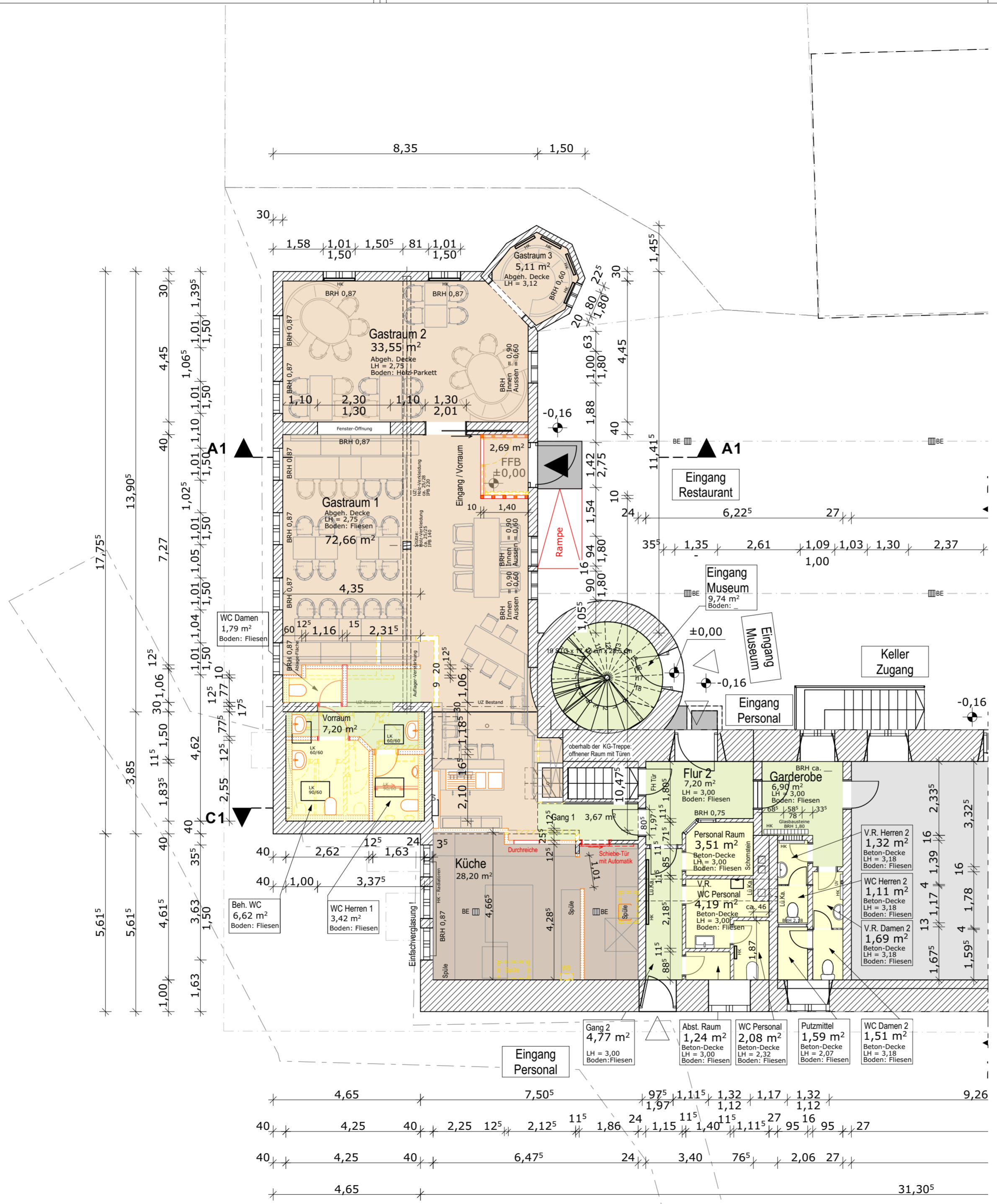
Gundriss Erdgeschoss - Restaurant
